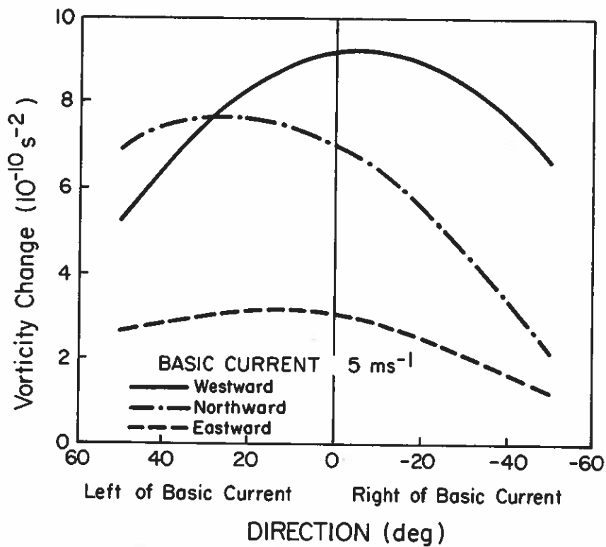
Fig. 11. As for Fig. 10 but for a basic current speed of 5 \text{ m s}^{-1} .
