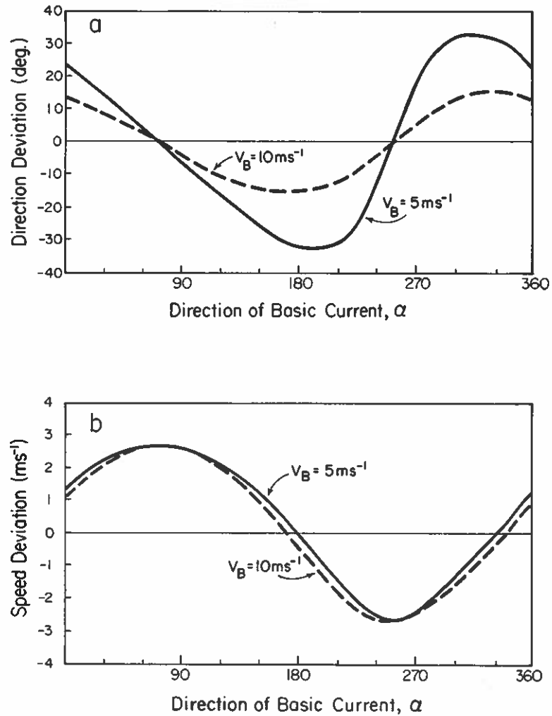
Fig. 6. Track (a) and speed (b) deviation from the basic flow for typical Northern Hemisphere cyclone parameters and two basic current speeds. A positive deviation means to the left of, and faster than the basic current.
