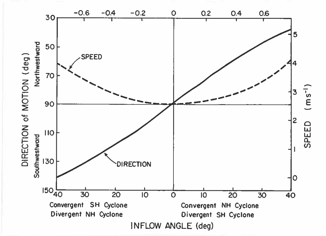
Fig. 2. The change in speed and direction of motion with degree of vergence in a tropical cyclone with no basic current.
