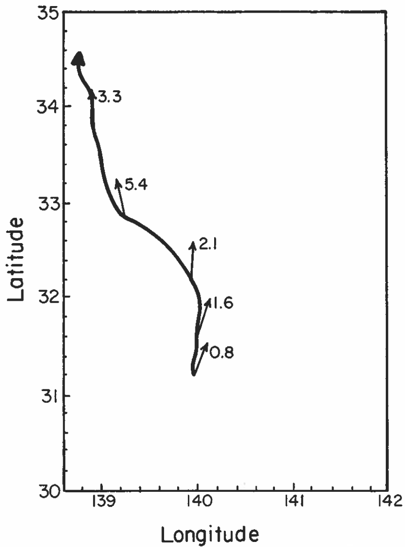
Fig. 9. Reconstruction of the trajectory (solid line) of a tropical cyclone from baroclinic experiment #1 of Kitade (1980). The arrows and numerals indicate the direction and speed ( \text{m s}^{-1} ) of the steering current at 10 hourly intervals.
