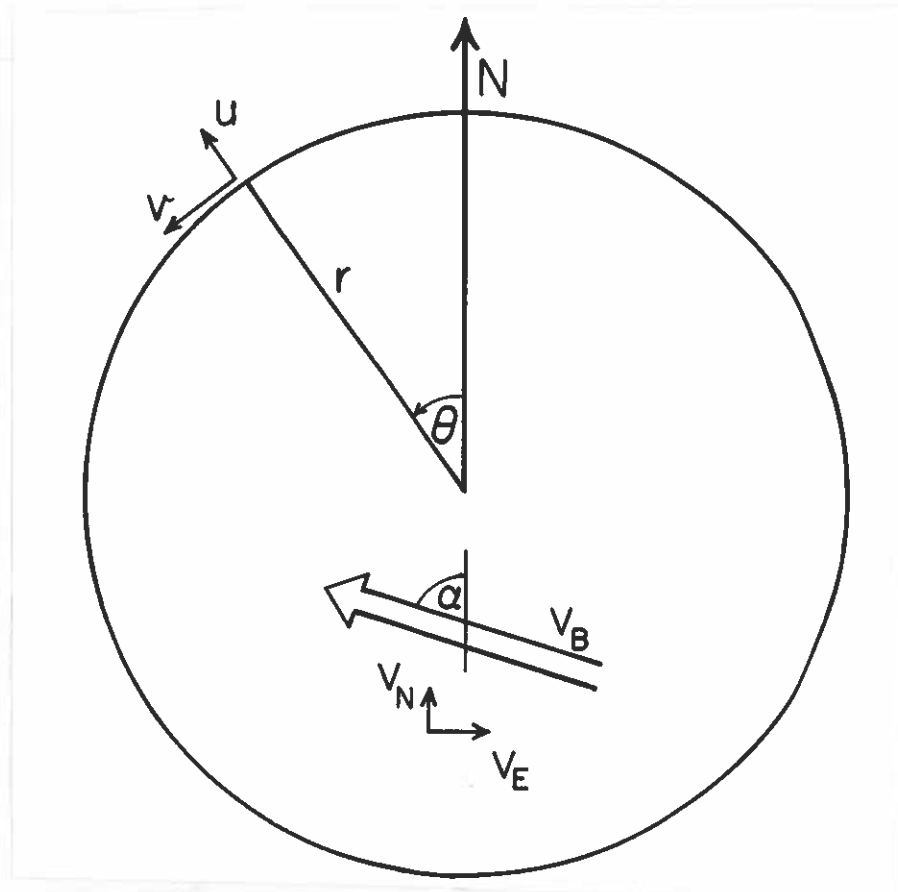
Fig. 1. The coordinate system used in this paper. The symbols are described in the text.
