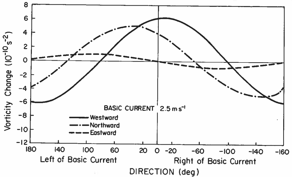
Fig. 10. Azimuthal variations of rate of vorticity change at the effective radius of 300 km for the typical cyclone described in section 3c and a basic current speed of 2.5 \text{ m s}^{-1} .
