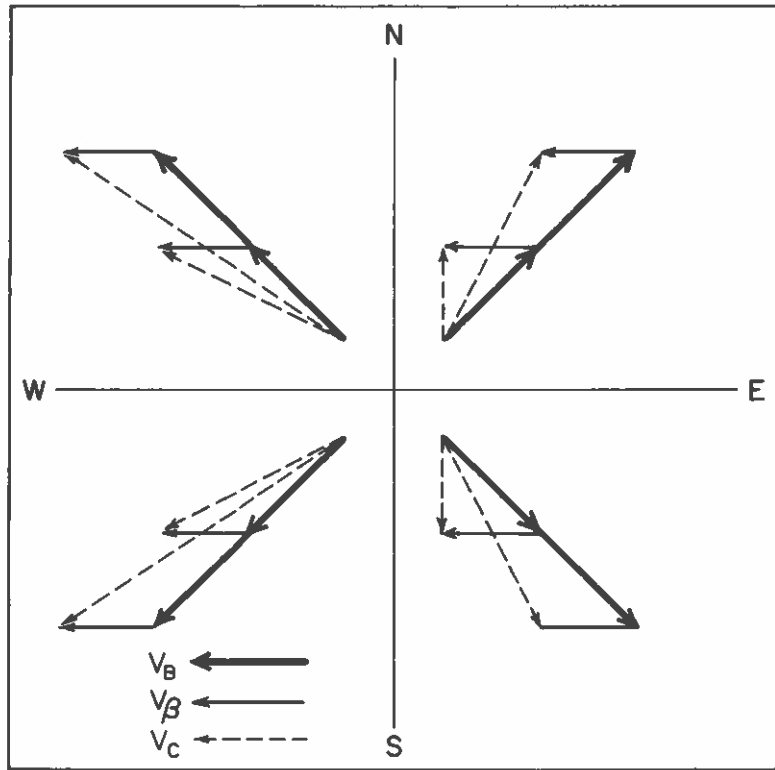
Fig. 5. A schematic illustration of the effects of adding a constant beta effect ( V_\beta ) to basic currents ( V_B ) of different directions and \beta speeds to produce a resultant cyclone motion ( V_C ).
