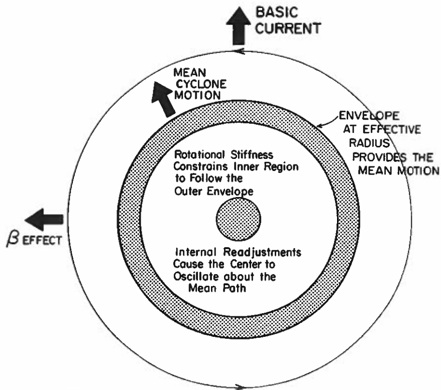
Fig. 7. A simple schematic of cyclone motion on a beta plane under a basic current.
