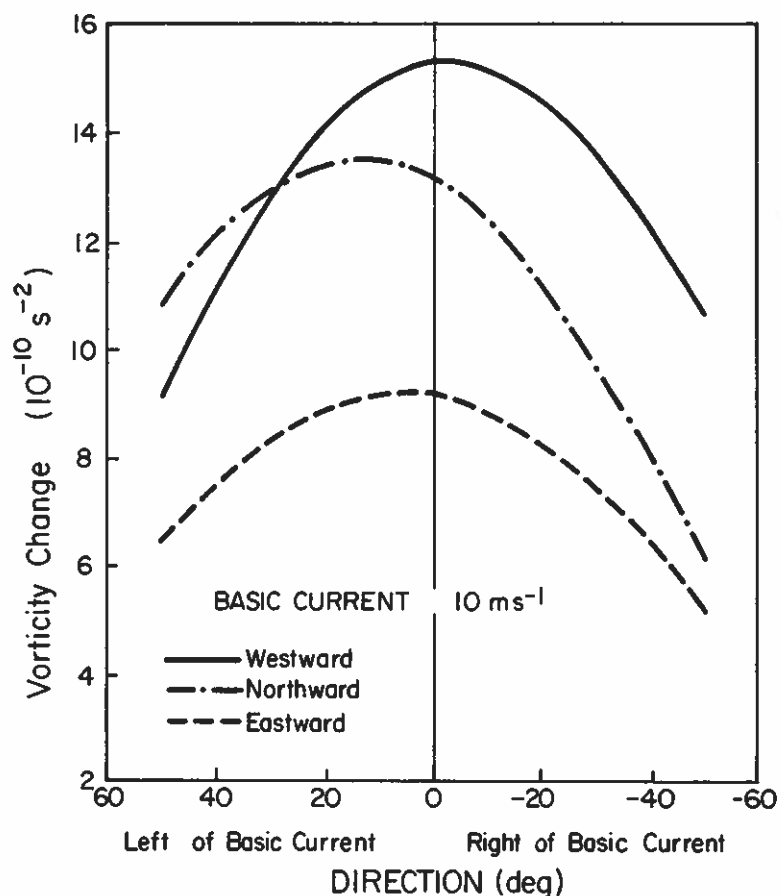
Fig. 12. As for Fig. 10 but for a basic current speed of 10 \text{ m s}^{-1} .
