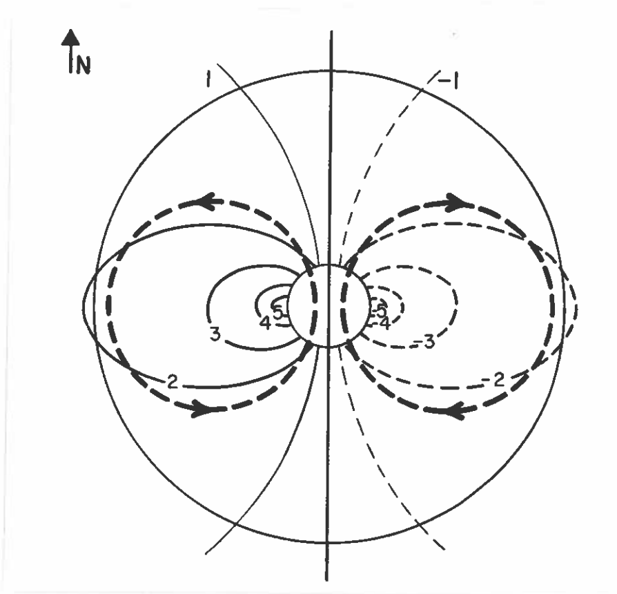
Fig. 3. Field of \partial\zeta/\partial t , in arbitrary units, centered on a symmetric, nonvergent Northern Hemispheric cyclone which is drifting westwards on a beta plane with no basic flow. Heavy dashed lines show the induced secondary circulation as a result of the vorticity changes.
