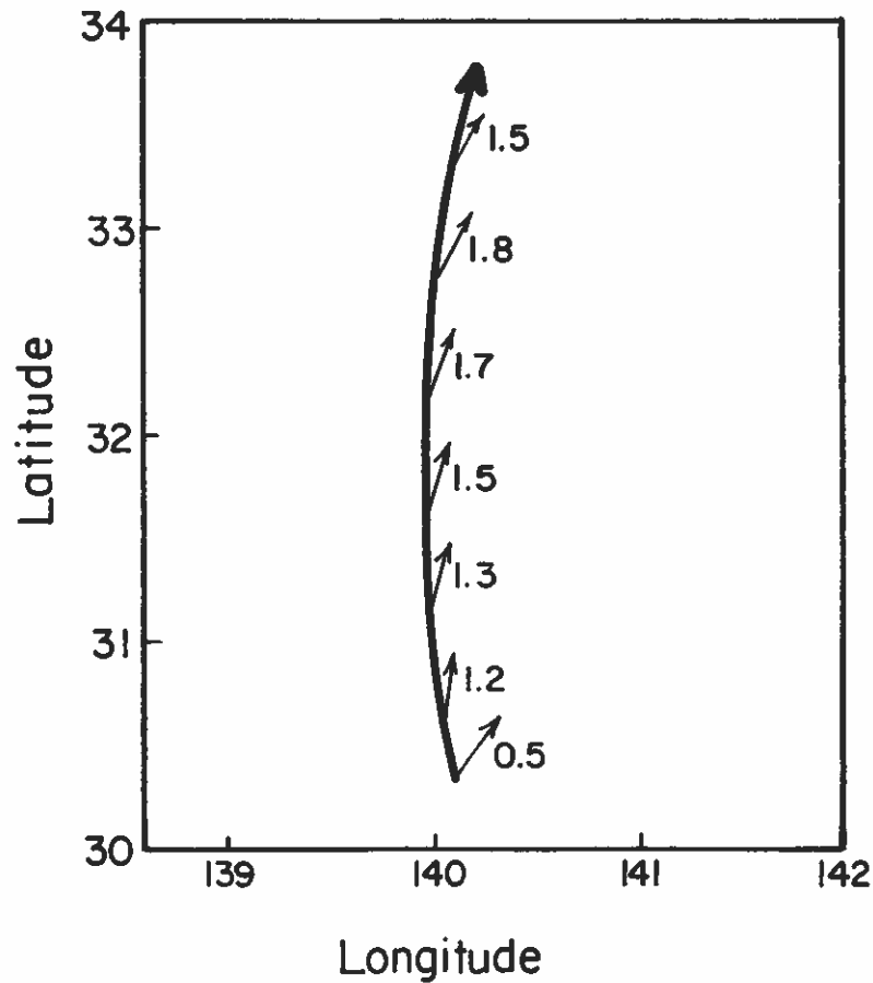
Fig. 4. Reconstruction of the trajectory of a tropical cyclone (heavy line) during an integration of a vergent quasi-barotropic model by Kitade (1980). The arrows and numerals indicate the direction and speed ( \text{m s}^{-1} ) of the steering current at 10 hourly intervals.
