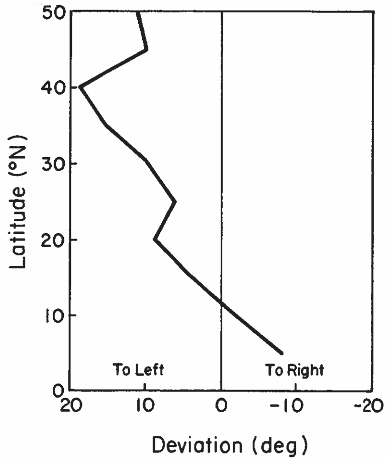
Fig. 8. Deviation of Northwest Pacific tropical cyclones from their geostrophic basic current (after Brand et al. , 1981).
