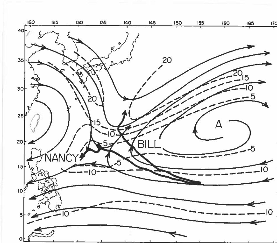
Fig. 13. Tracks of idealized typhoons Bill and Nancy relative to a constant basic state field of motion.
